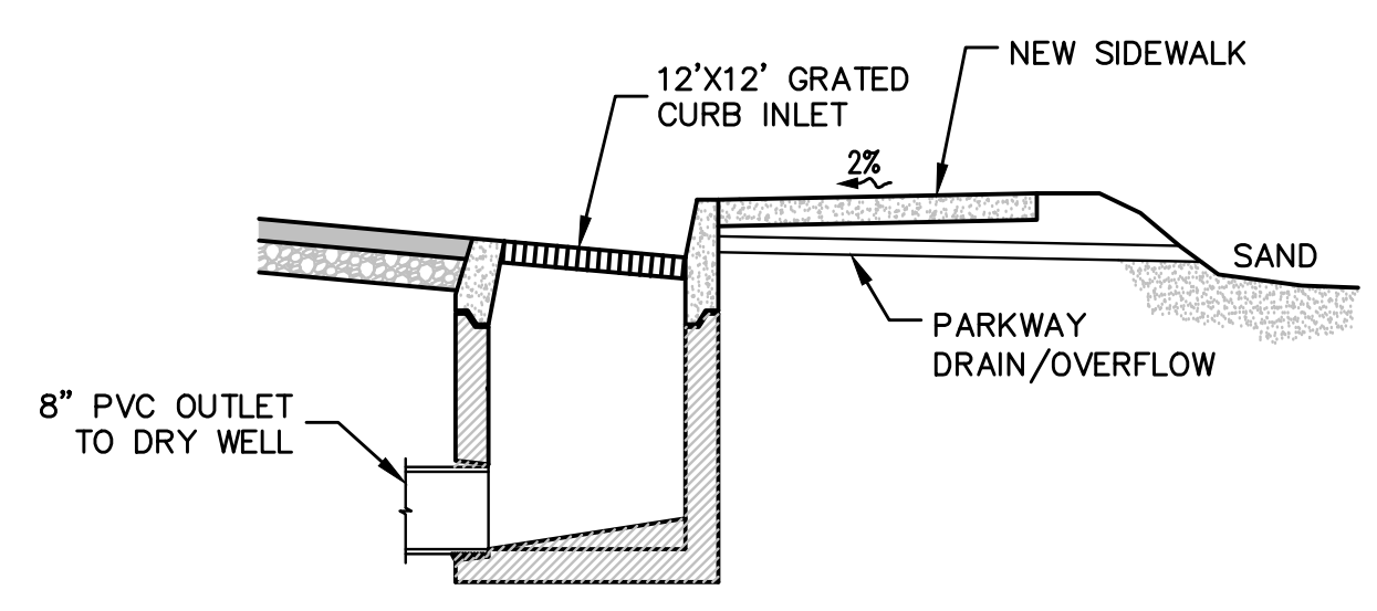
STORM DRAIN GRATE INLET
