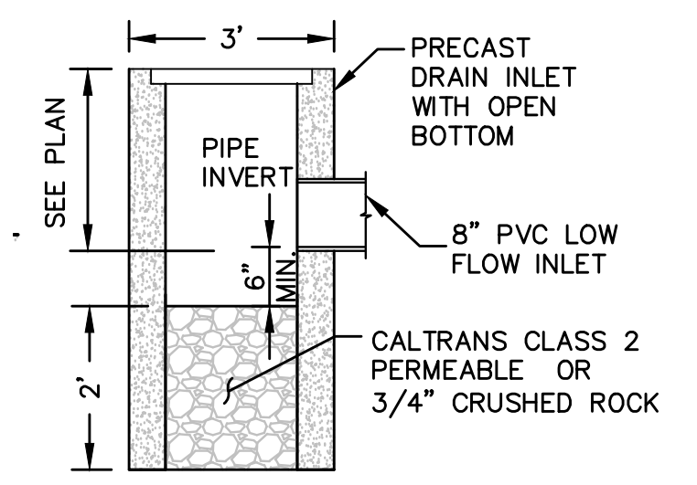
DRY WELL
